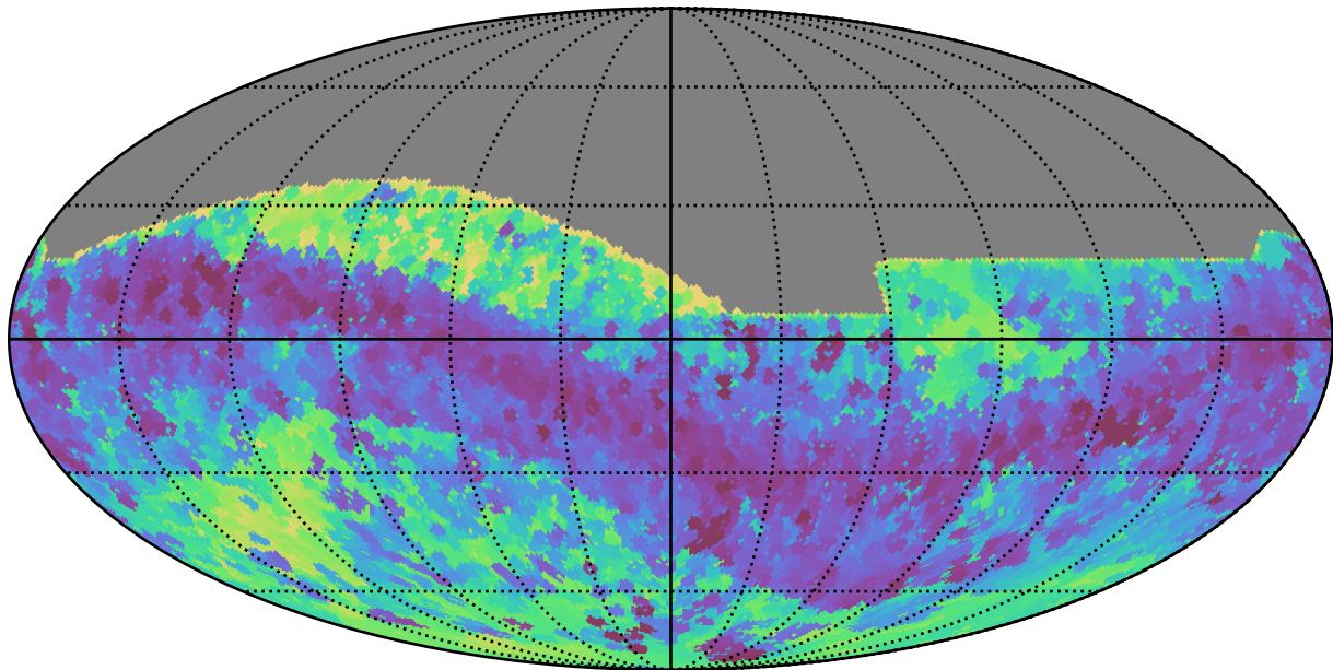
baseline_v3.2_10yrs All sky all bands: Min skyBrightness
