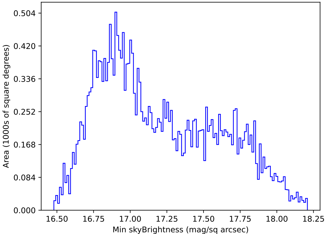
baseline_v3.2_10yrs All sky all bands: Min skyBrightness
