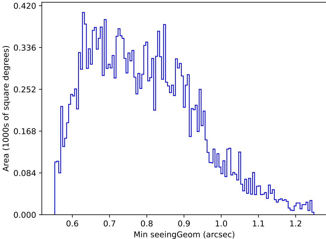
baseline_v3.2_10yrs Yr 1 u band: Min seeingGeom
