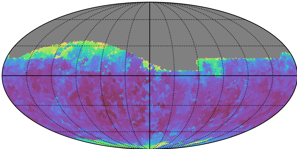
baseline_v3.2_10yrs Yr 1 r band: Min seeingGeom
