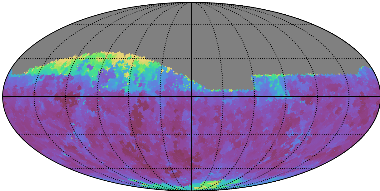
baseline_v3.2_10yrs Yr 1 i band: Min seeingGeom
