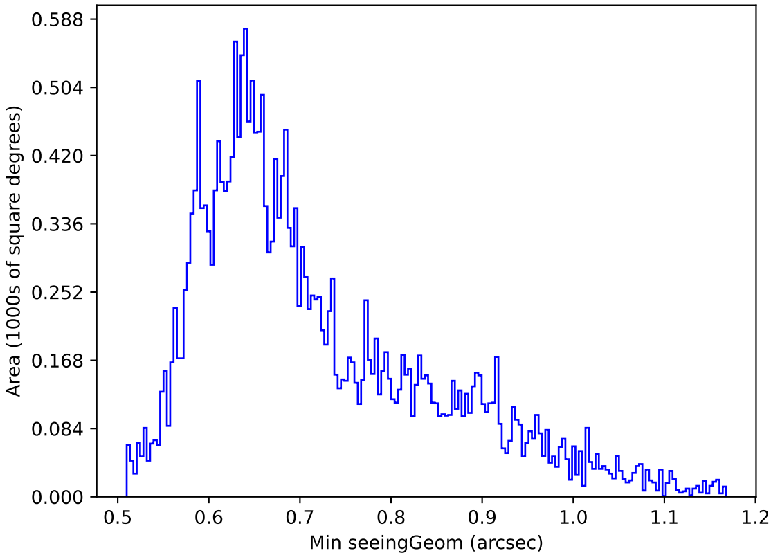
baseline_v3.2_10yrs Yr 1 g band: Min seeingGeom
