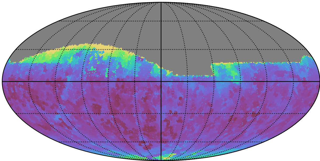
baseline_v3.2_10yrs Yr 1 all bands: Min seeingGeom
