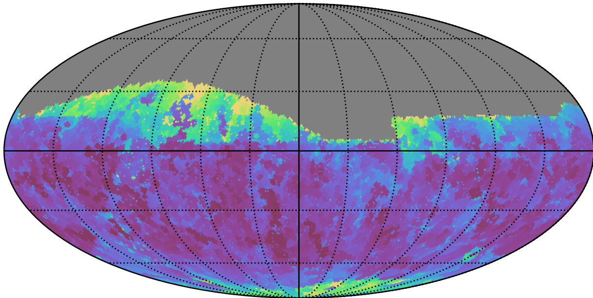
baseline_v3.2_10yrs Yr 1 z band: Min seeingEff
