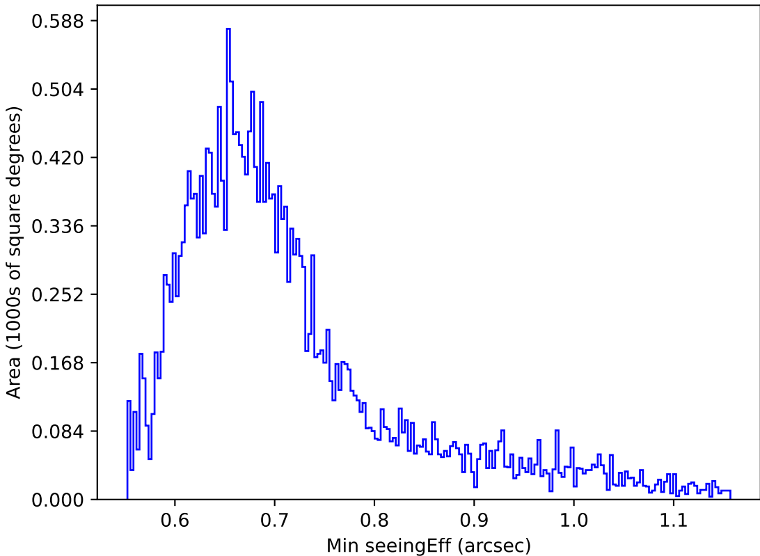
baseline_v3.2_10yrs Yr 1 z band: Min seeingEff
