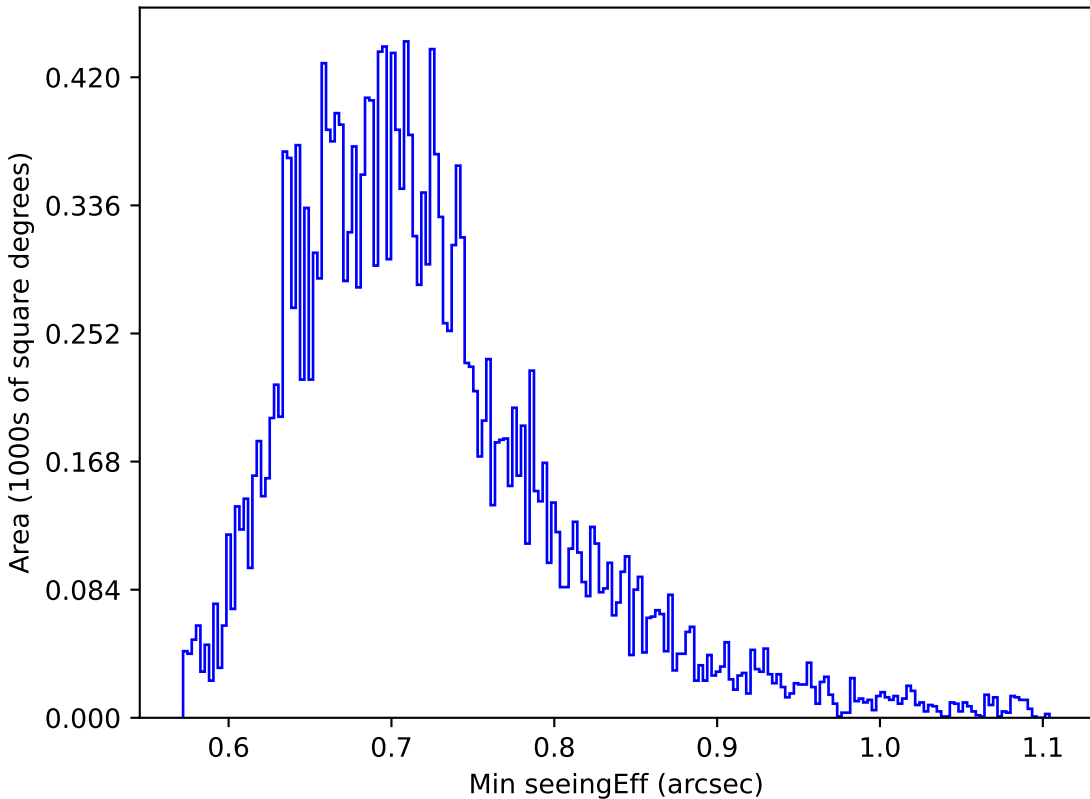
baseline_v3.2_10yrs Yr 1 y band: Min seeingEff
