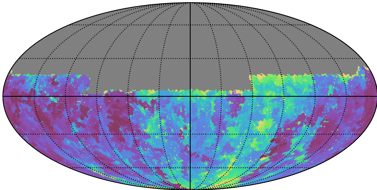
baseline_v3.2_10yrs Yr 1 u band: Min seeingEff
