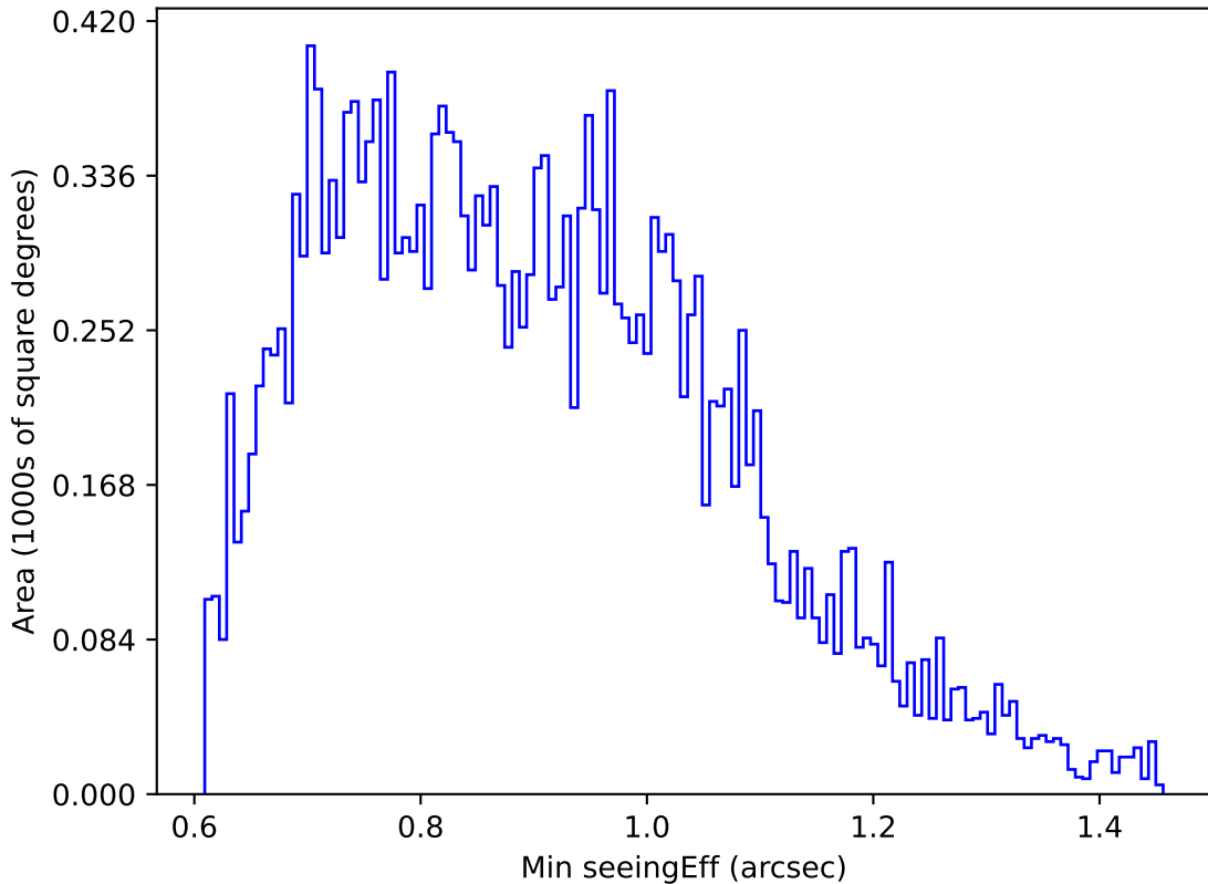
baseline_v3.2_10yrs Yr 1 u band: Min seeingEff
