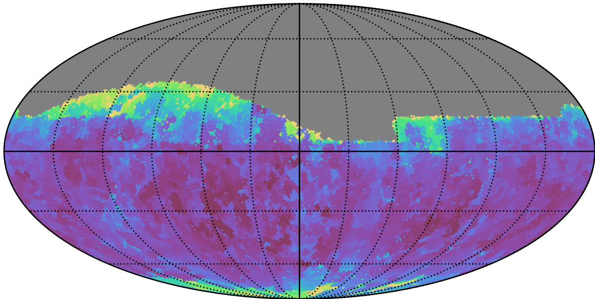
baseline_v3.2_10yrs Yr 1 r band: Min seeingEff
