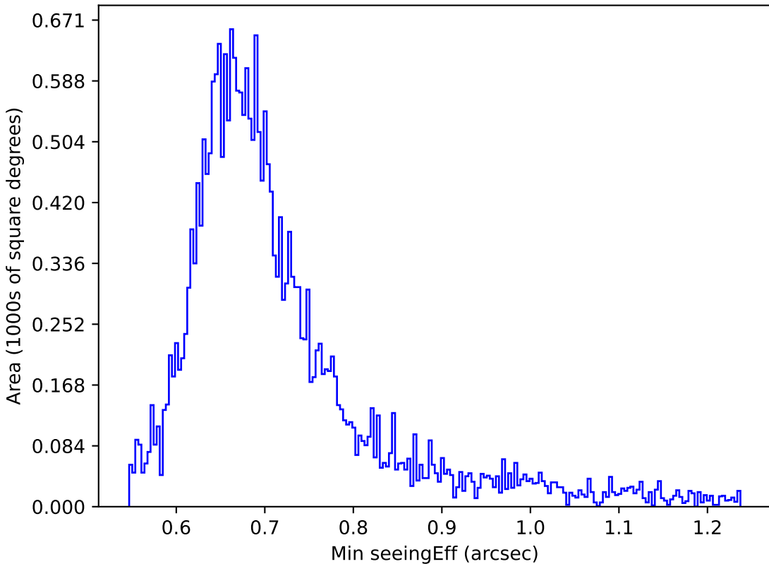
baseline_v3.2_10yrs Yr 1 r band: Min seeingEff
