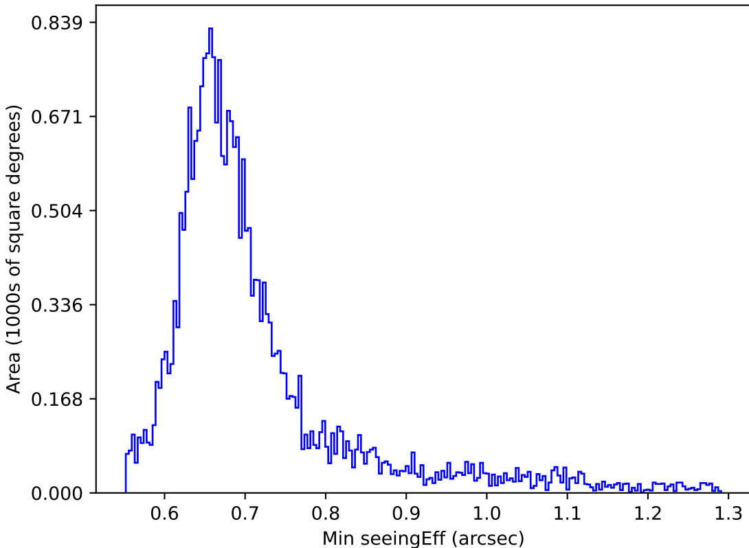
baseline_v3.2_10yrs Yr 1 i band: Min seeingEff
