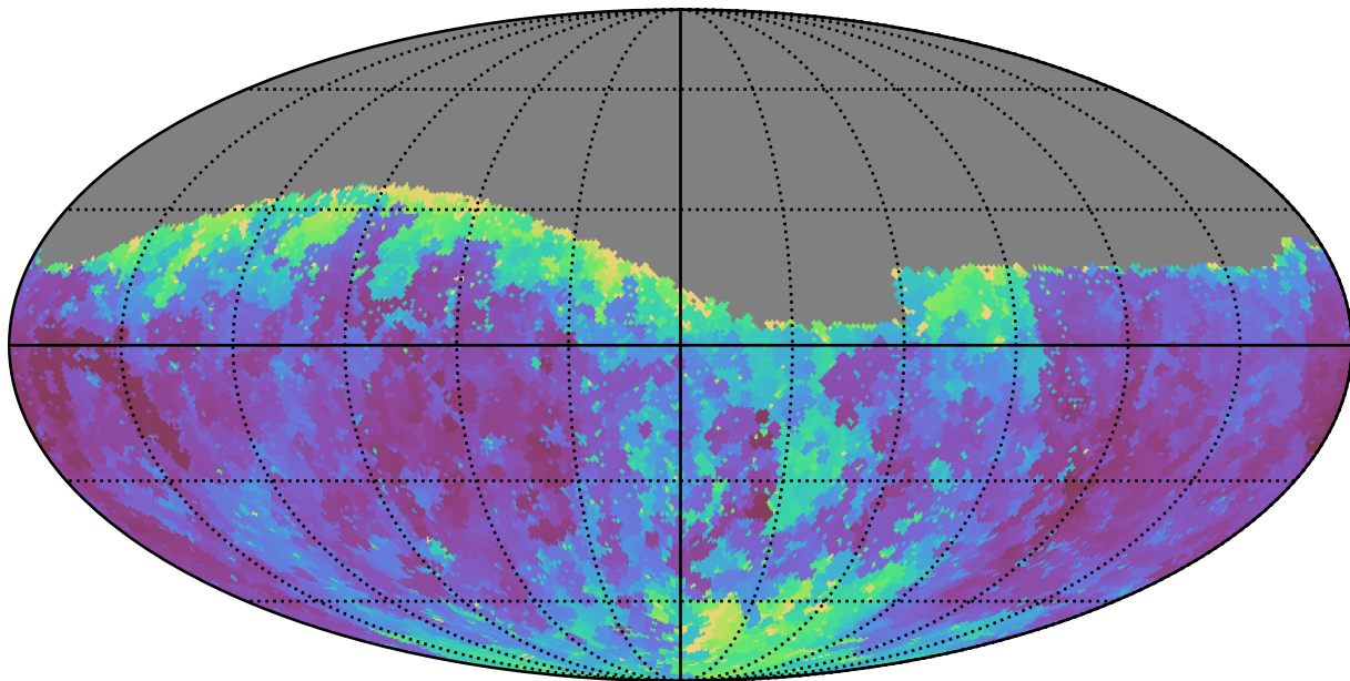
baseline_v3.2_10yrs Yr 1 g band: Min seeingEff
