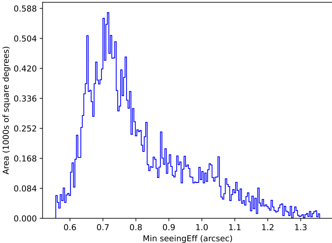
baseline_v3.2_10yrs Yr 1 g band: Min seeingEff
