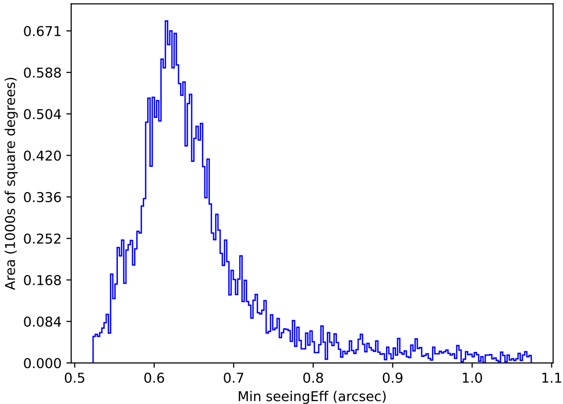
baseline_v3.2_10yrs Yr 1 all bands: Min seeingEff
