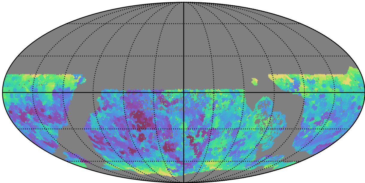
baseline_v3.2_10yrs WFD z band: Min seeingEff
