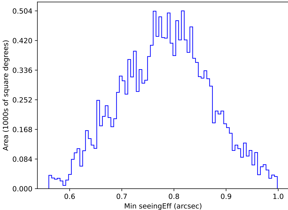
baseline_v3.2_10yrs WFD u band: Min seeingEff
