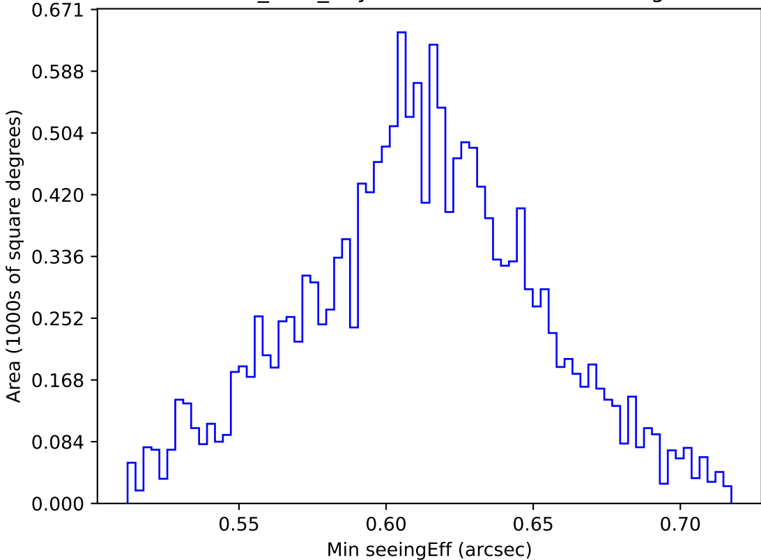
baseline_v3.2_10yrs WFD r band: Min seeingEff
