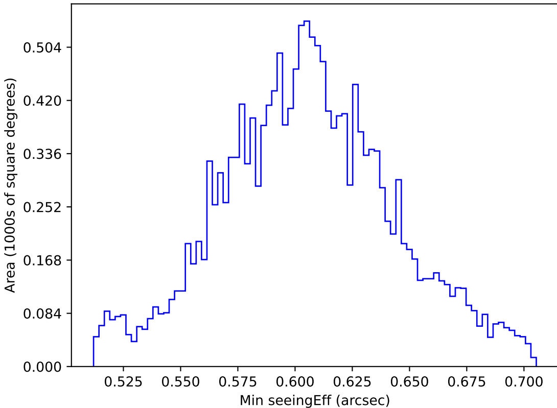
baseline_v3.2_10yrs WFD i band: Min seeingEff
