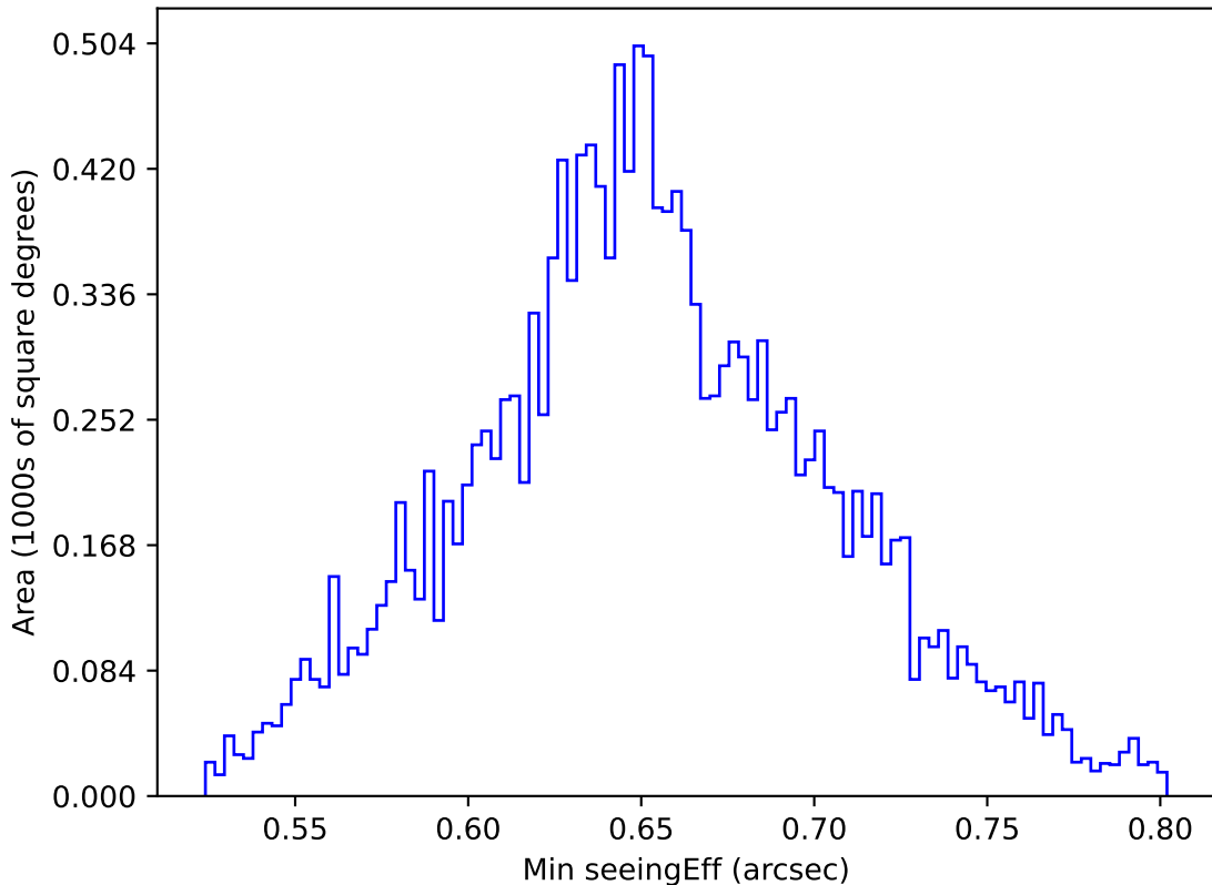
baseline_v3.2_10yrs WFD g band: Min seeingEff
