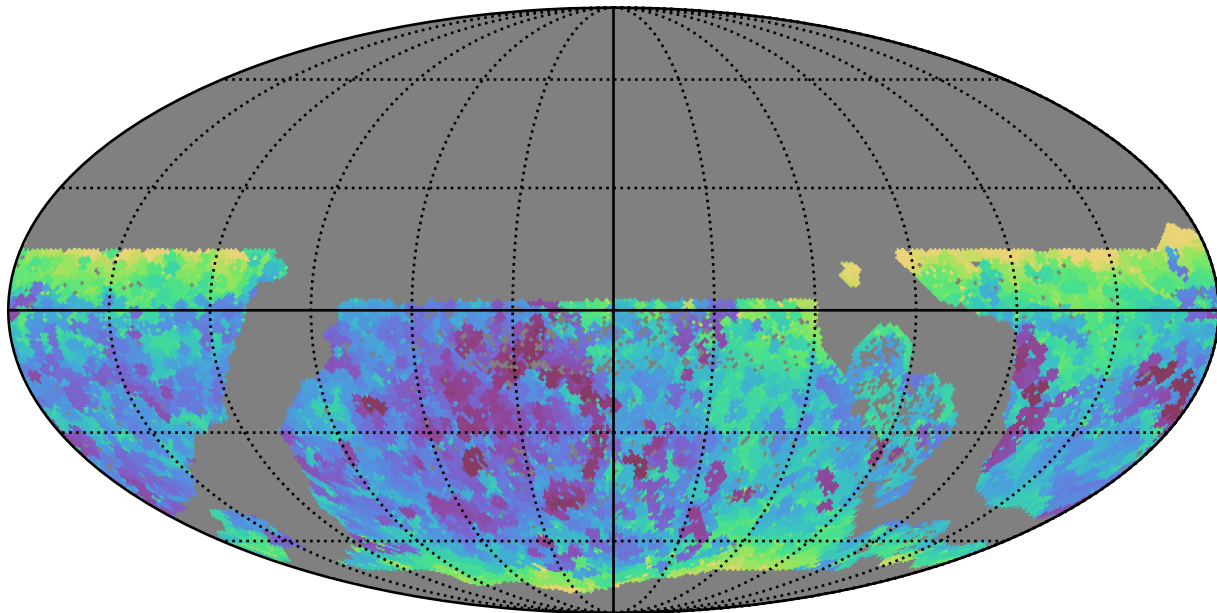
baseline_v3.2_10yrs WFD all bands: Min seeingEff
