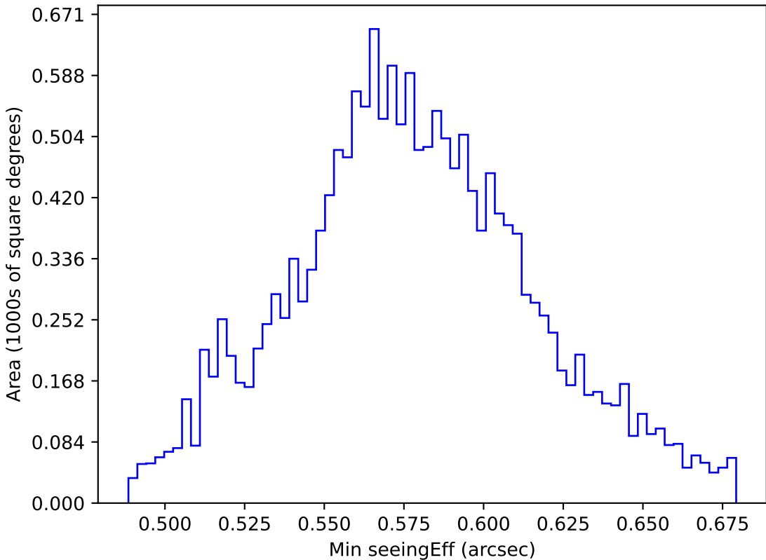
baseline_v3.2_10yrs WFD all bands: Min seeingEff
