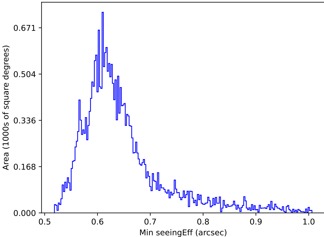
baseline_v3.2_10yrs All sky z band: Min seeingEff
