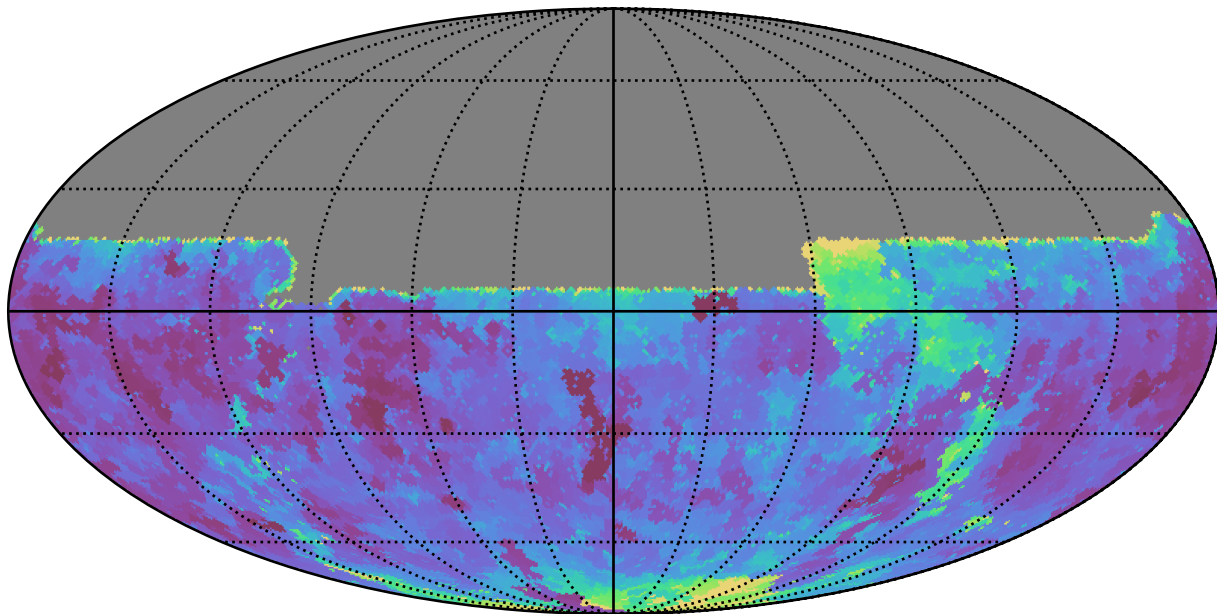
baseline_v3.2_10yrs All sky u band: Min seeingEff
