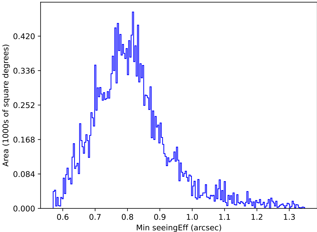
baseline_v3.2_10yrs All sky u band: Min seeingEff
