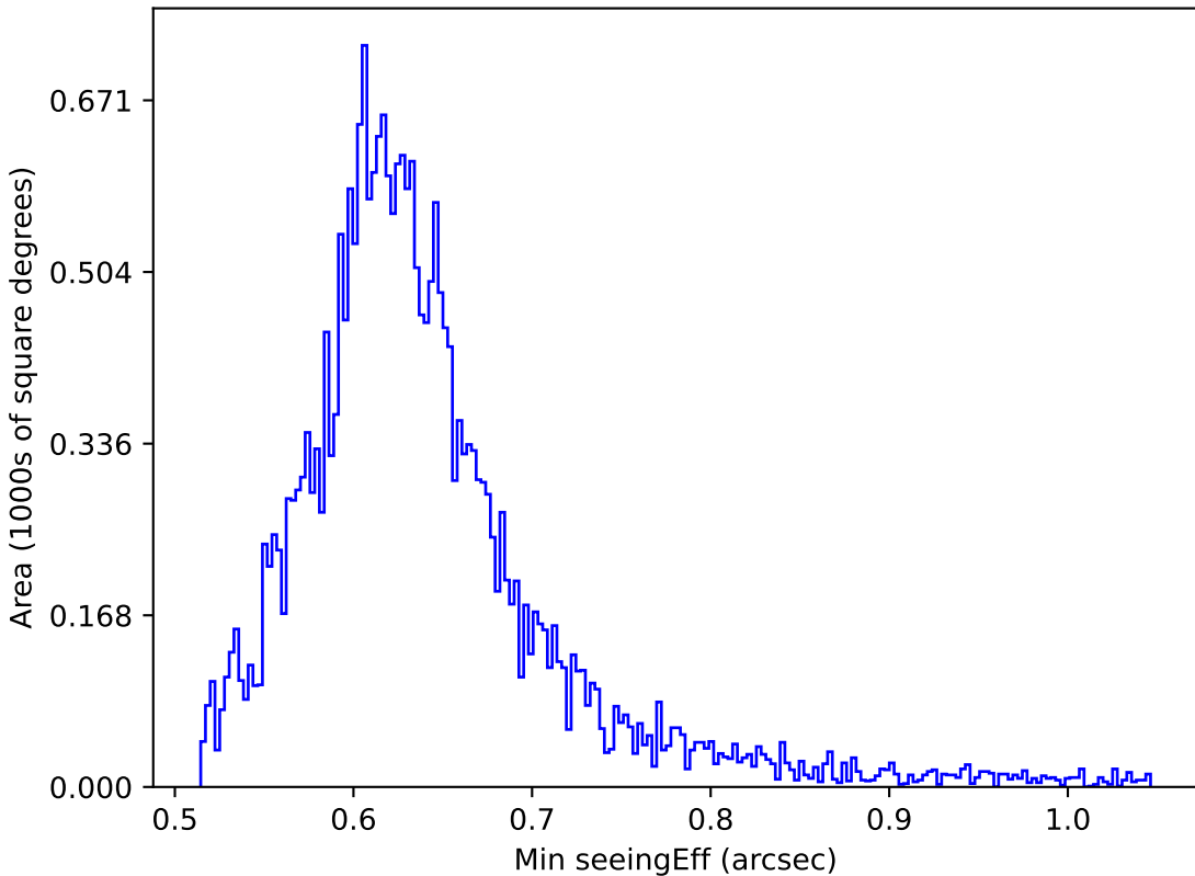
baseline_v3.2_10yrs All sky r band: Min seeingEff
