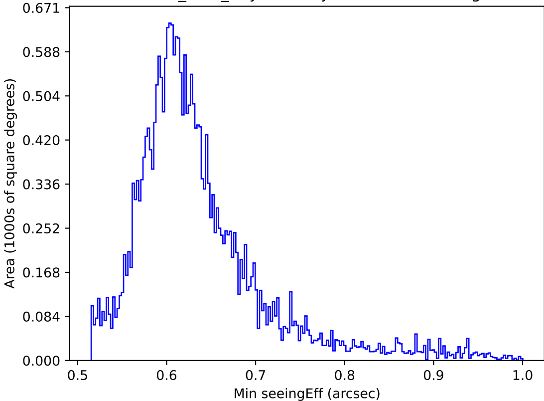
baseline_v3.2_10yrs All sky i band: Min seeingEff
