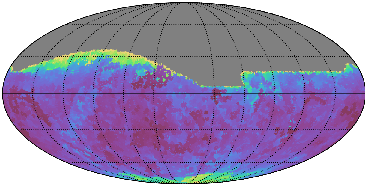
baseline_v3.2_10yrs All sky g band: Min seeingEff
