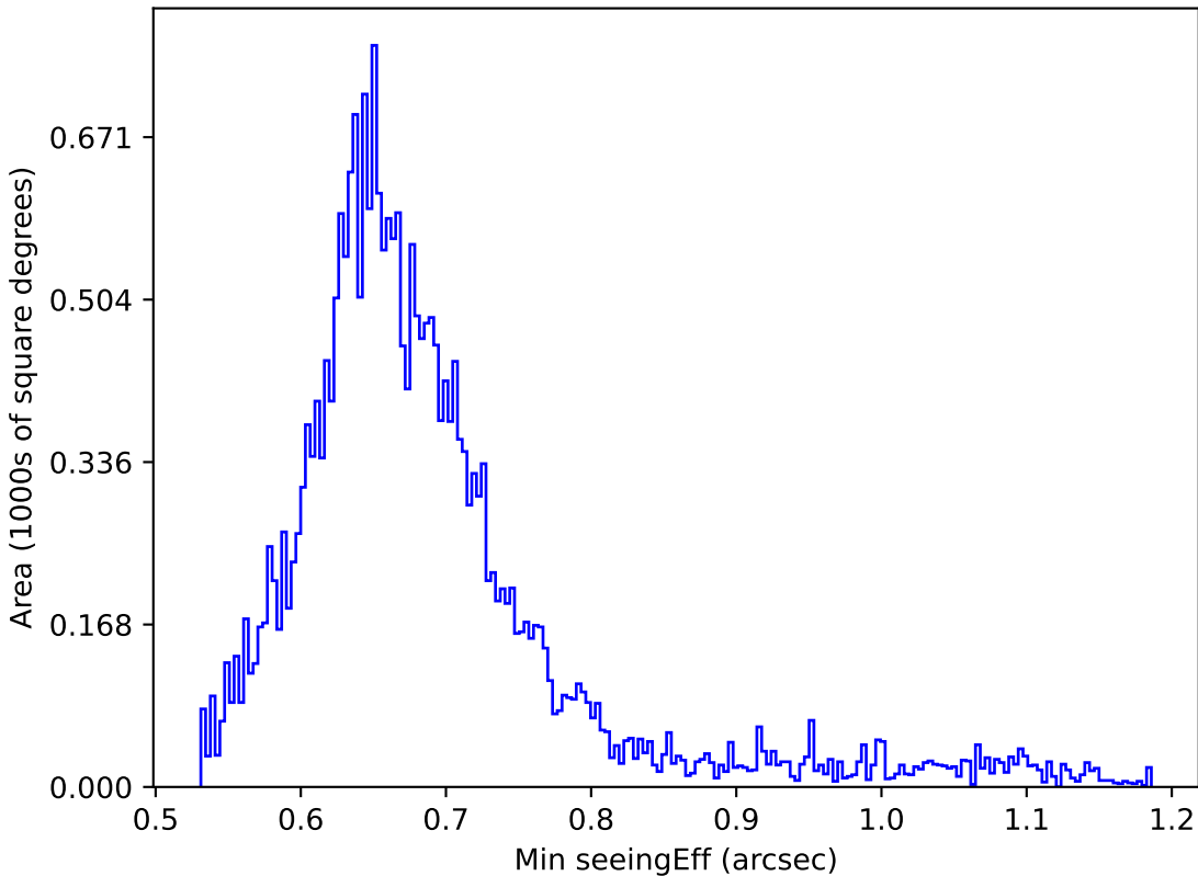
baseline_v3.2_10yrs All sky g band: Min seeingEff
