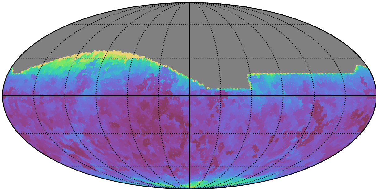
baseline_v3.2_10yrs All sky all bands: Min seeingEff
