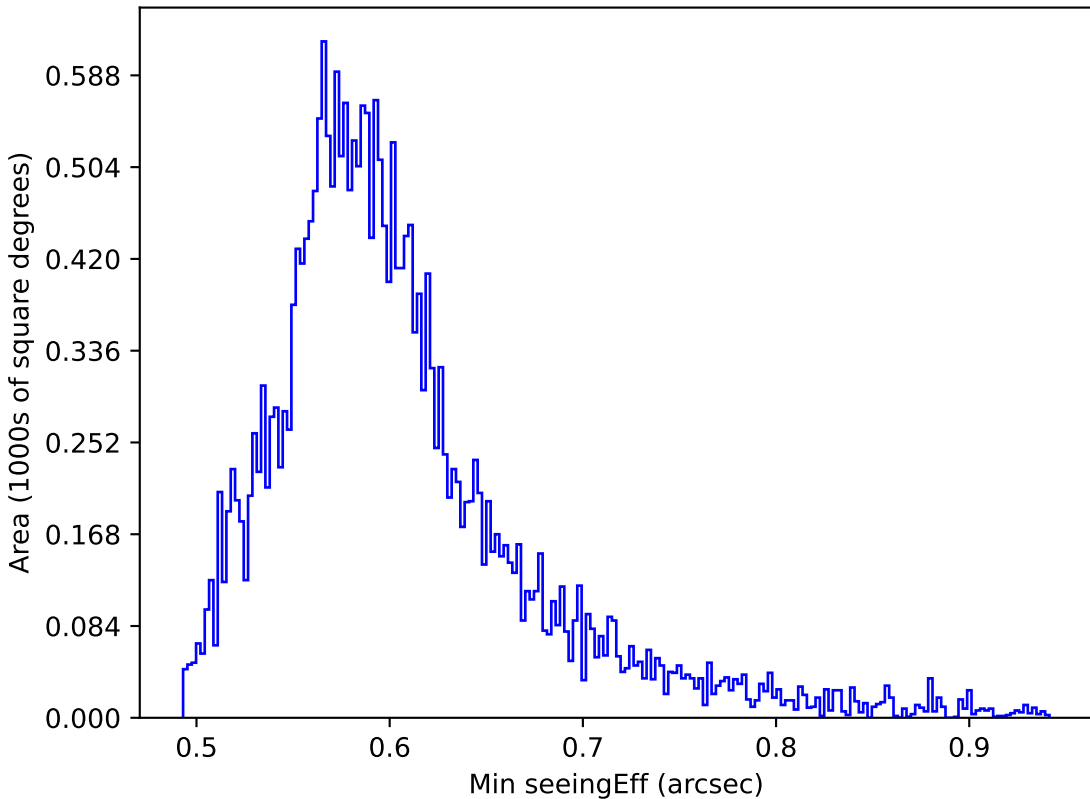
baseline_v3.2_10yrs All sky all bands: Min seeingEff
