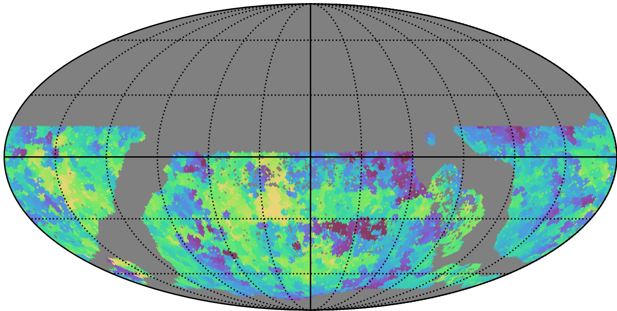
baseline_v3.2_10yrs WFD u band: Min saturation_mag
