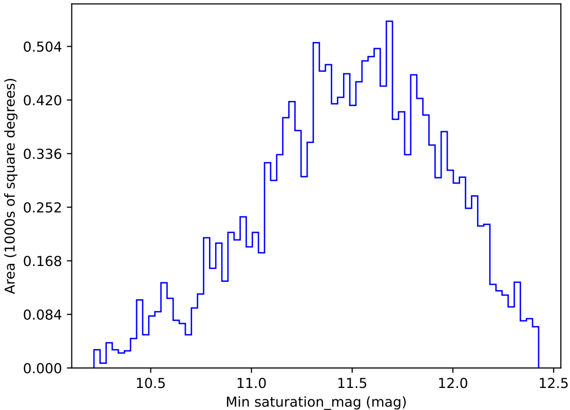
baseline_v3.2_10yrs WFD u band: Min saturation_mag
