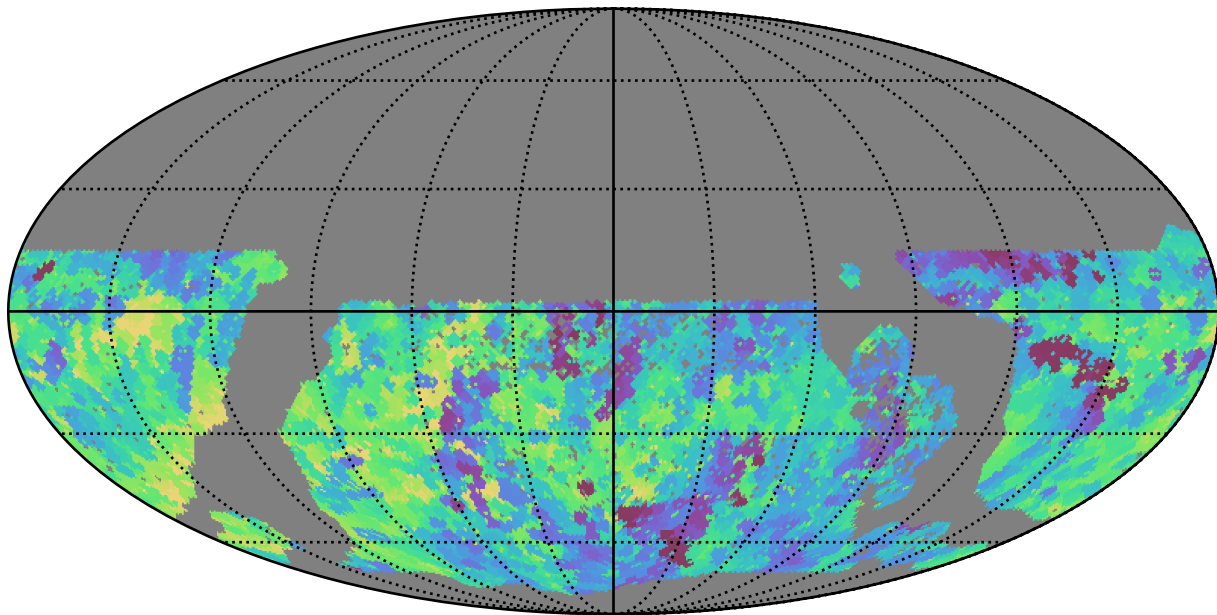
baseline_v3.2_10yrs WFD r band: Min saturation_mag
