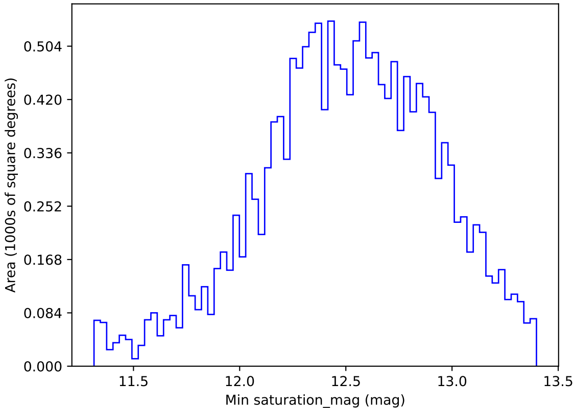
baseline_v3.2_10yrs WFD r band: Min saturation_mag
