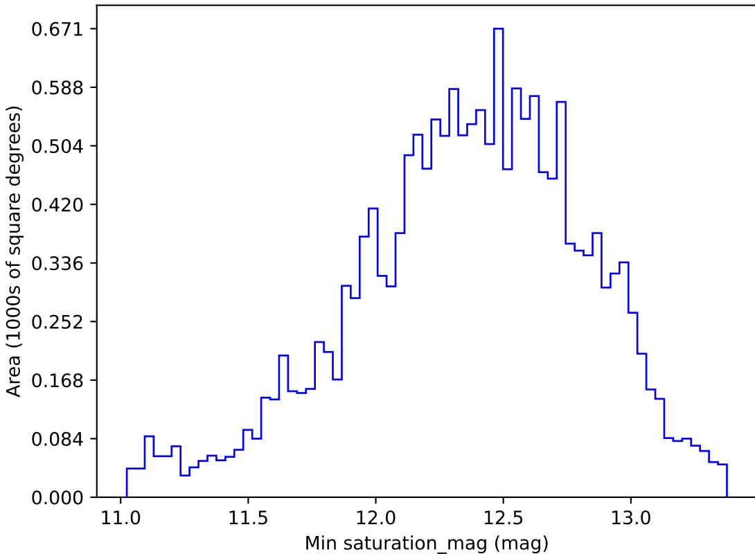
baseline_v3.2_10yrs WFD i band: Min saturation_mag
