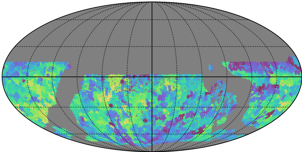
baseline_v3.2_10yrs WFD g band: Min saturation_mag
