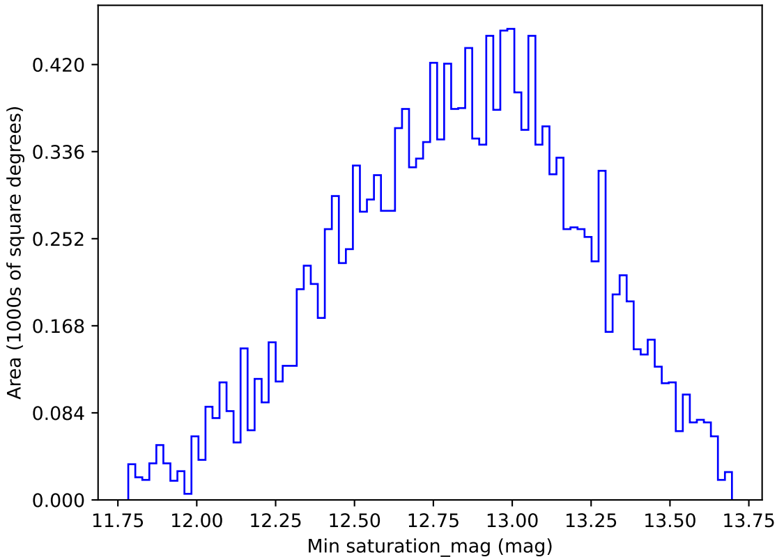
baseline_v3.2_10yrs WFD g band: Min saturation_mag
