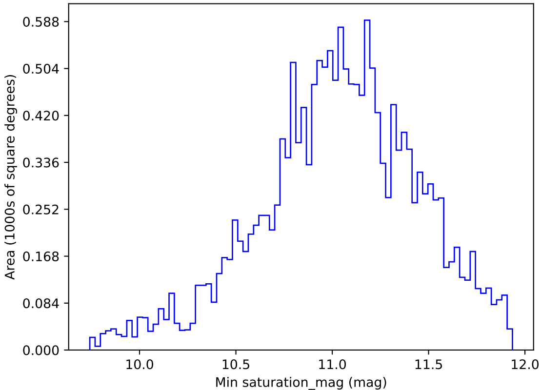
baseline_v3.2_10yrs WFD all bands: Min saturation_mag
