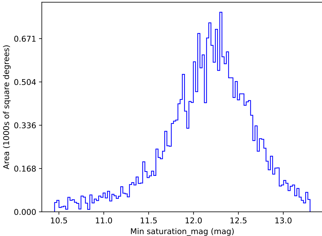
baseline_v3.2_10yrs All sky z band: Min saturation_mag
