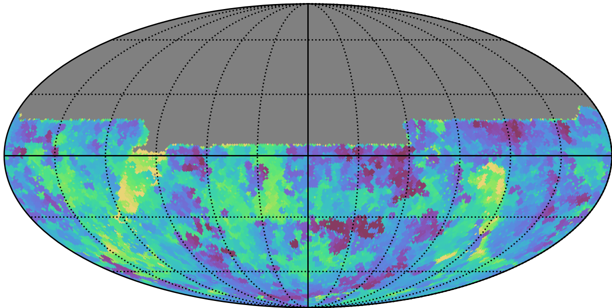
baseline_v3.2_10yrs All sky u band: Min saturation_mag
