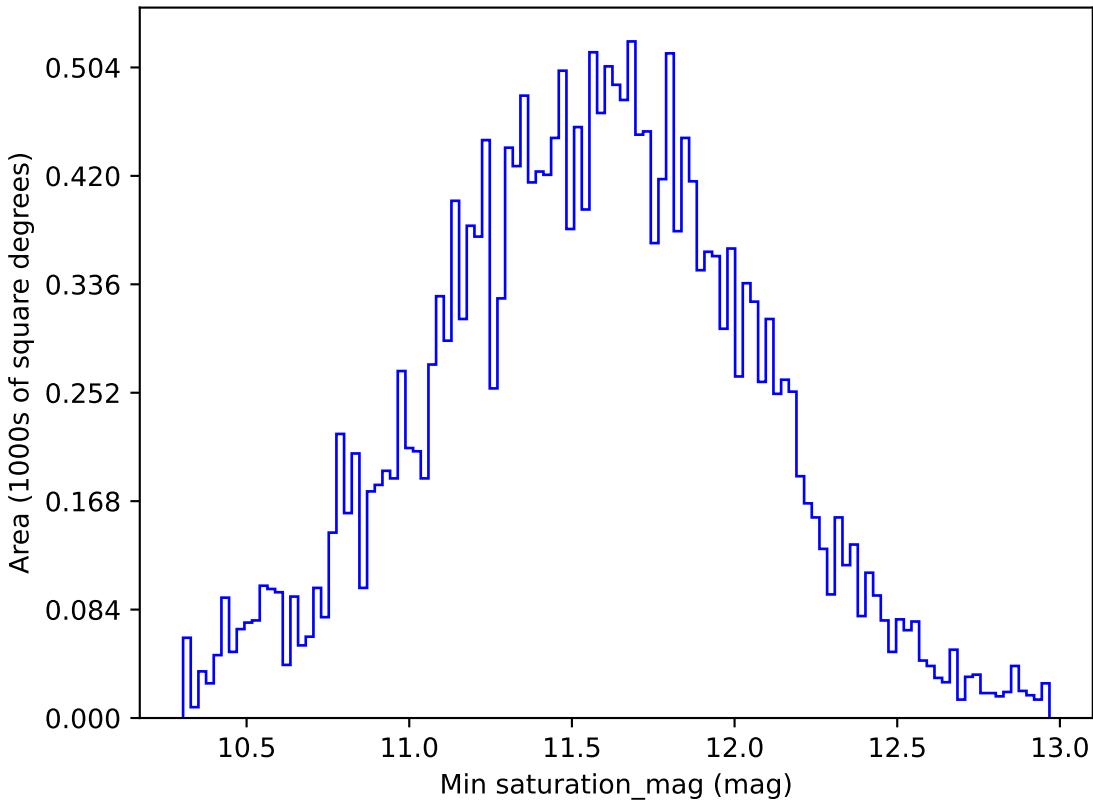
baseline_v3.2_10yrs All sky u band: Min saturation_mag
