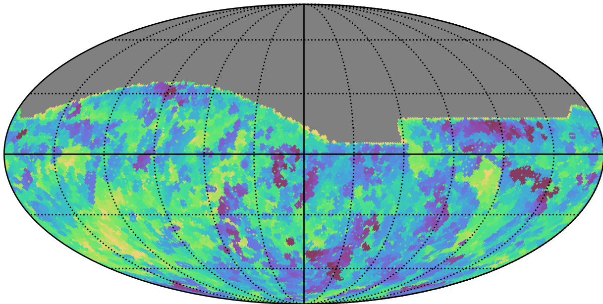
baseline_v3.2_10yrs All sky r band: Min saturation_mag
