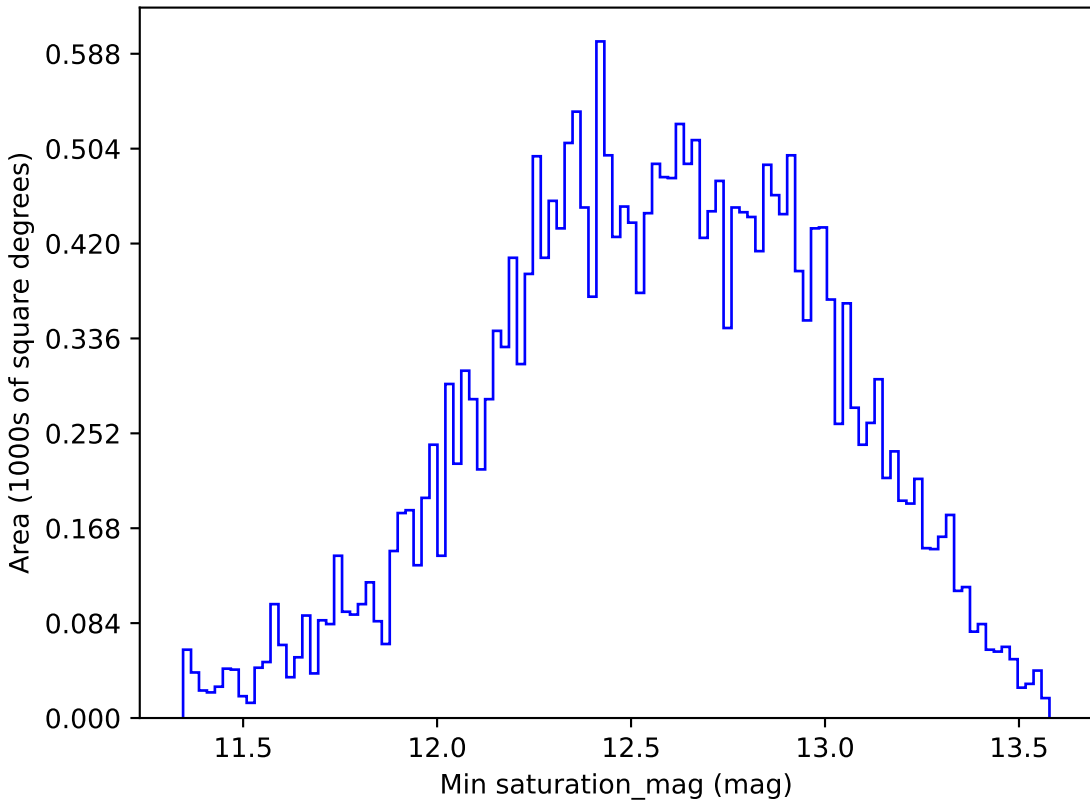
baseline_v3.2_10yrs All sky r band: Min saturation_mag
