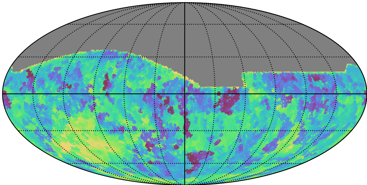
baseline_v3.2_10yrs All sky i band: Min saturation_mag
