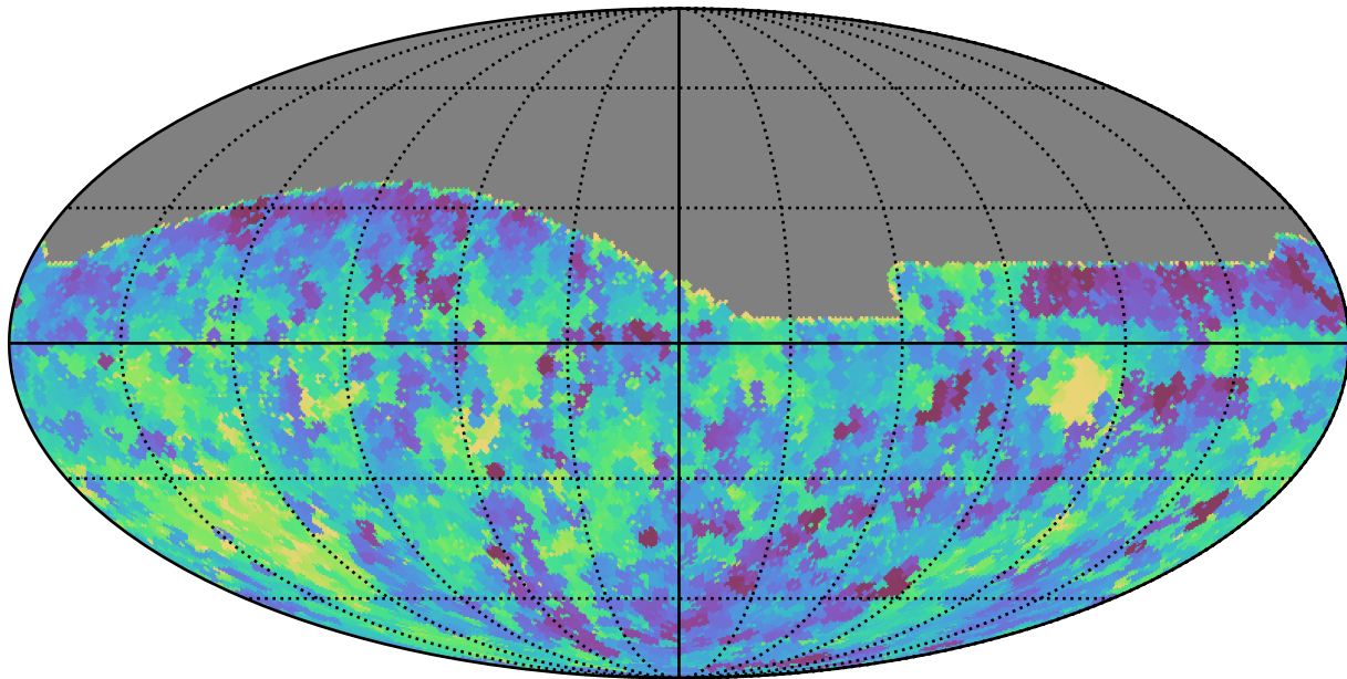
baseline_v3.2_10yrs All sky g band: Min saturation_mag
