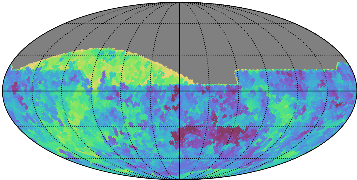
baseline_v3.2_10yrs All sky all bands: Min saturation_mag
